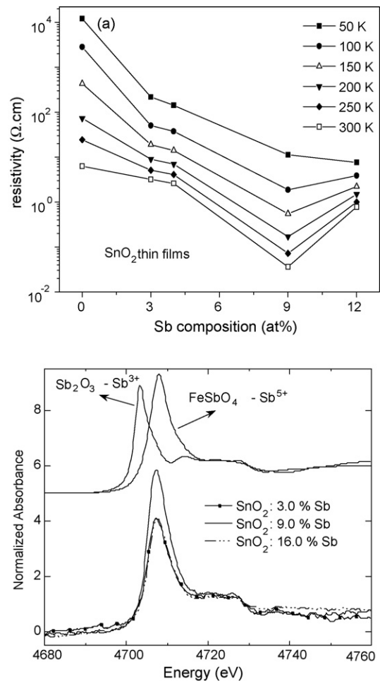
Fig. 1. (a) Resistivity as function of Sb doping in \text{SnO}_2 thin films, measured at several temperatures (lines are drawn only as a guide to the eyes). (b) XANES data for reference compounds and Sb-doped \text{SnO}_2 thin films. \text{Sb}_2\text{O}_3 presents oxidation state \text{Sb}^{3+} and \text{FeSbO}_4 , oxidation state \text{Sb}^{5+} .
